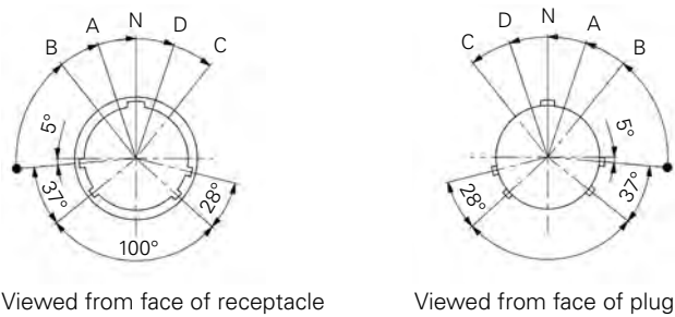
Viewed from face of receptacle
